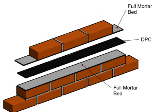
Figure 2 – DPC bedding
